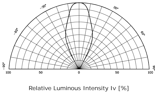
Fig. 5 Radiation Diagram
