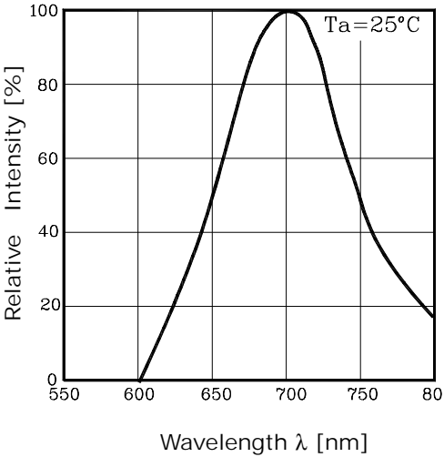
Fig. 4 Spectrum Distribution
