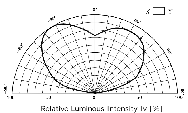
Fig. 5-2 Radiation Diagram(Y)
