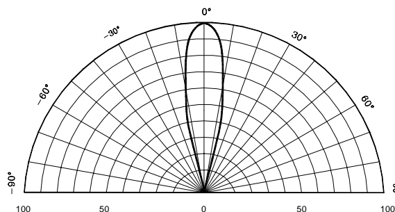
Fig. 5 Radiation Diagram
